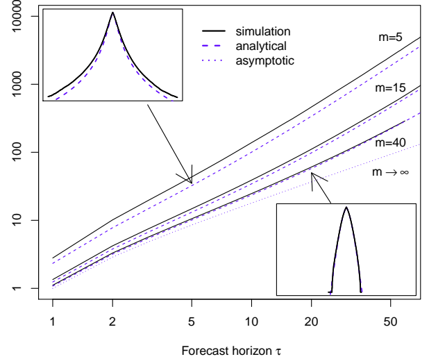
Figure 12: Error growth for large simulations of an IMA(1,1) process, to check Eq. (14) and (15). Simulations are done using 5000 time series of 100 periods, all with with \mu = 0.04 , K = 0.05 , \theta = 0.6 . The insets show the distribution of forecast errors, as in Fig. 8, for m = 5, 40
